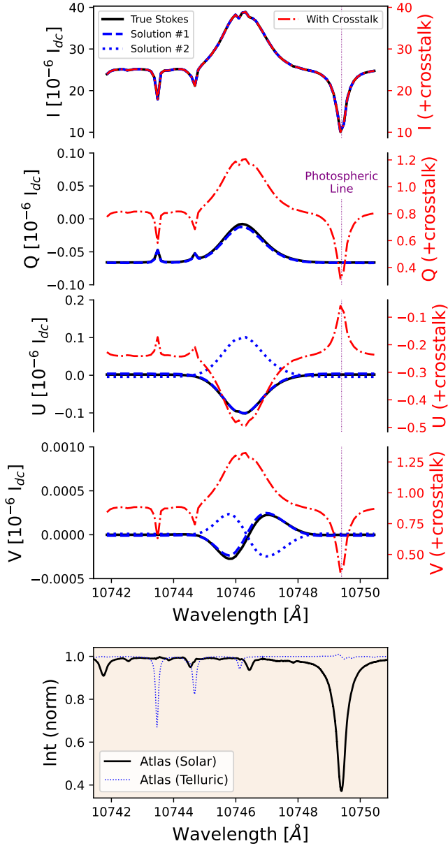
Figure 7. (top four panels) The true synthetic Stokes vector emergent from the MHD simulation at \langle x, z \rangle = \langle 32, 32 \rangle Mm is given in black. Dashdot red lines represent the ‘measured’ Stokes vector with polarized crosstalk added, while the blue lines show the two solutions found for the crosstalk corrected signals. The right axis tick marks apply only to the crosstalk added signals. (bottom panel) The photospheric atlas spectrum acquired at disk center separated into solar and telluric components.
