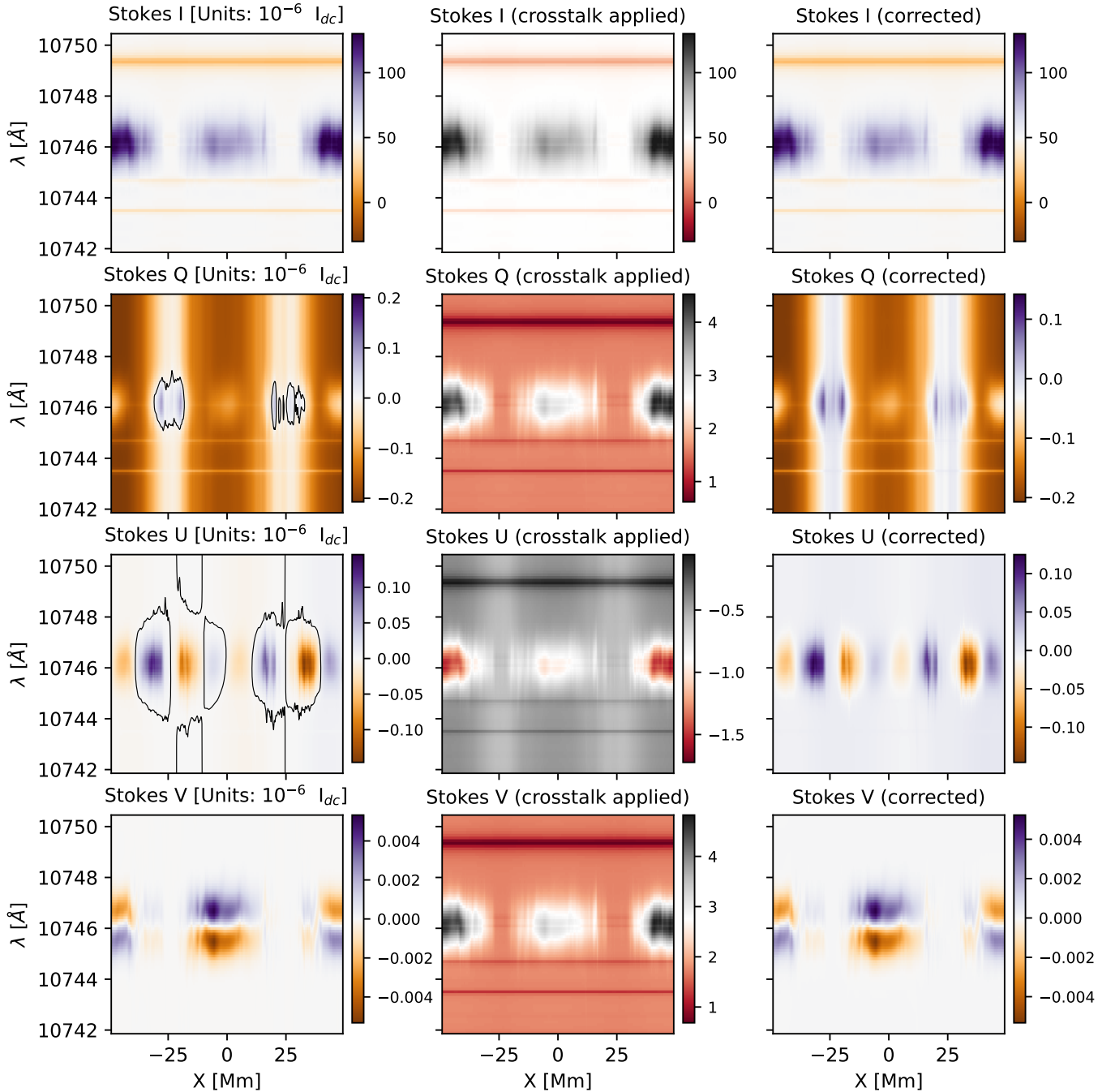
Figure 8. Synthetic Stokes spectra centered on the Fe XIII 10746 Å line including Thomson scattering and an unpolarized background spectrum. The Stokes spectra incident on the optical system at a simulation height of Z = 30 Mm are shown on the left. Zero-level contours for Q and U are provided to distinguish regions where Stokes U takes negative or positive values. The middle column shows the Stokes spectra with crosstalk applied. The right column shows spectra after applying the crosstalk correction method.
