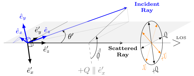
Figure 1. Geometry of the Thomson scattering calculation referenced to a fixed Stokes frame along the line-of-sight (LOS) defined by the scattering direction and with Stokes +Q aligned parallel to the \hat{e}'_x polarization vector of the scattered ray.
