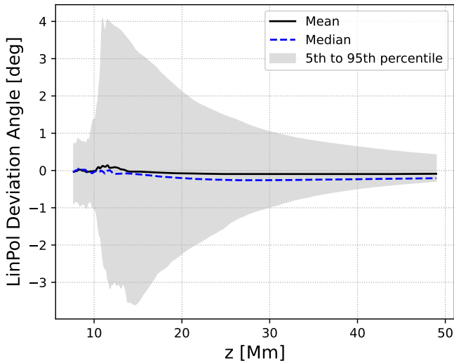
Figure 6. Height dependence of the linear polarization deviation angle relative to the tangential direction for the synthetic Thomson scattered signals shown in Figure 5.
