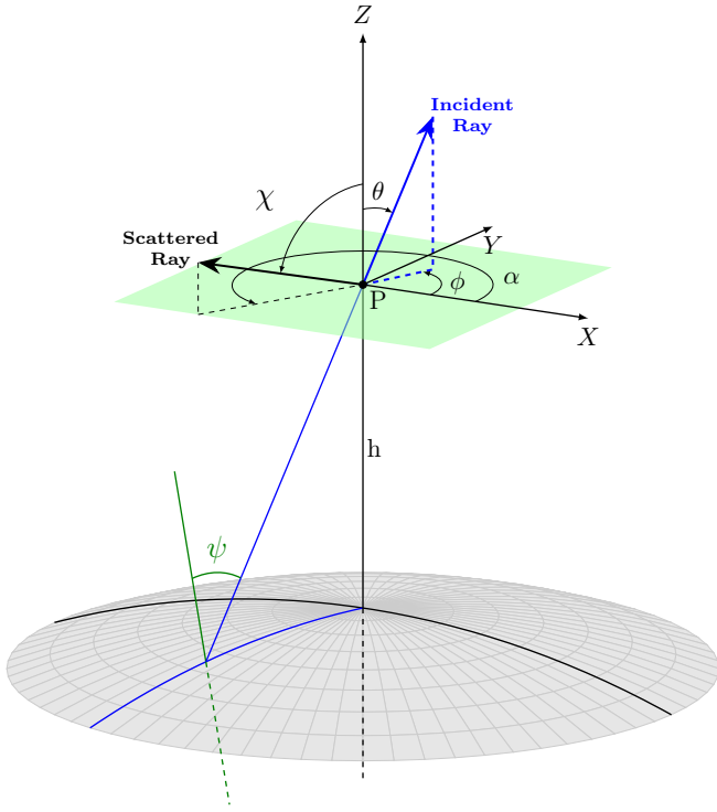
Figure 2. Geometry for the line-of-sight (LOS) frame relative to the axes used for quantifying the radiation field in the local radial frame. The LOS frame is specified by the zyz extrinsic Euler angles \gamma = 0 (not shown), \beta = \chi and \alpha = \alpha . The choice \gamma = 0 results in the +Q Stokes direction being aligned with the projected radial direction at point P, which is located at height h above the stellar surface. One example incident ray is shown in blue, which exits the stellar photosphere at an angle \psi relative to the surface normal.
