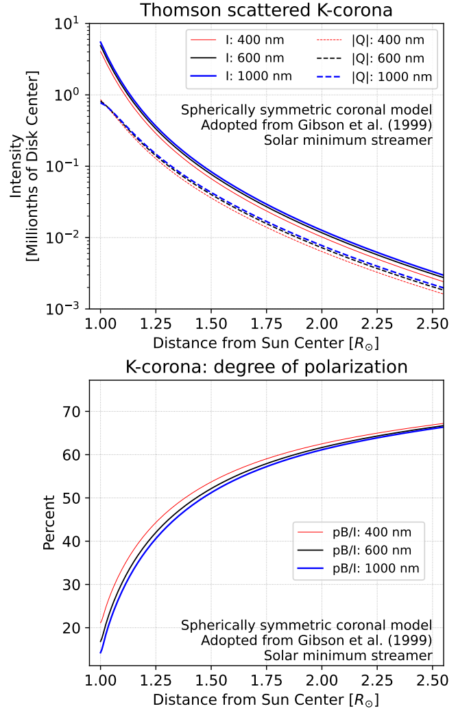
Figure 3. (top) Forward synthesized Thomson scattered K-corona intensity and the absolute value of Stokes Q for a spherically symmetric electron density model and cylindrically symmetric incident radiation field. (bottom) The corresponding degree of polarization.
