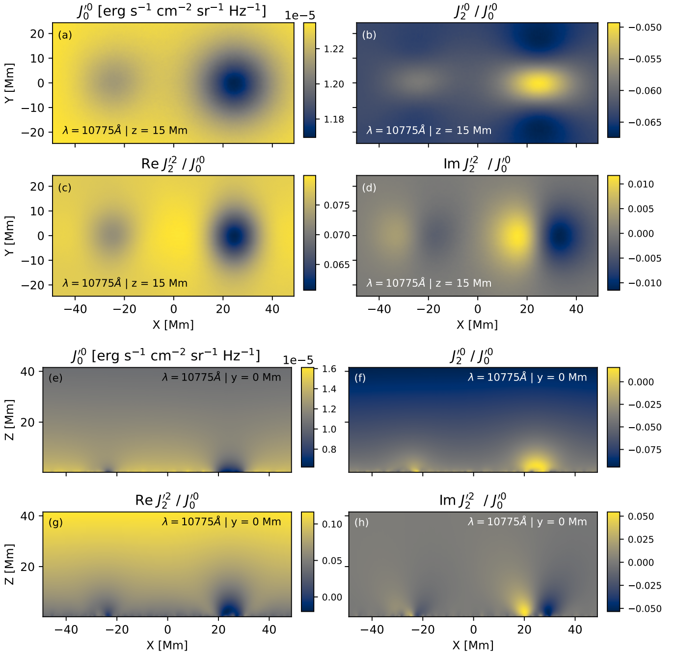
Figure 4. The incident radiation field components within the bipolar 3D MURaM coronal simulation that contribute to the Thomson scattered continuum at \lambda = 10775 \text{ \AA} . The observer’s line-of-sight aligns with the Y axis, and for reference, two simulated sunspots are located near X \pm 25 \text{ Mm} ( Y = 0 \text{ Mm} ). The top panels (a-d) provide a horizontal slice at Z = 15 \text{ Mm} , and the bottom panels (e-h) show a vertical slice at Y = 0 \text{ Mm} . Note the total mean intensity ( J_0^0 ) is given in spectral radiance units while each other panel is normalized by J_0^0 .
