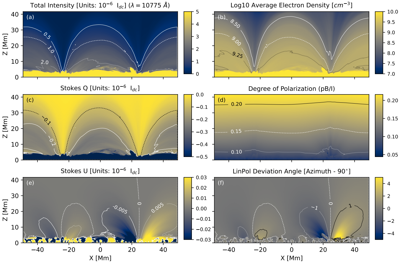
Figure 5. Synthesized polarized Thomson scattered continuum along the -y direction through the bipolar MHD coronal simulation. Panels a,c,e show the total intensity, Stokes Q, and Stokes U intensities in units of millionths of the disk center spectral radiance. Panel b is the line-of-sight average electron density in the simulation domain. Panel d shows the degree of polarization while panel f shows the deviation angle of the linear polarization direction relative to the tangential direction, which in the establish reference frame is equal to the azimuth (-0.5 \arctan 2(U, Q)) minus 90 degrees.
